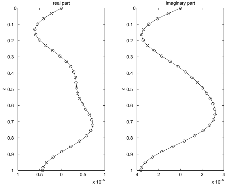
Figure 2: A comparison of the back-scattered waves calculated with step size h = 1/8 (small circles) and h = 1/128 (solid line).
