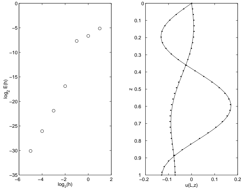
Figure 1: (a). Relative errors of u(L, z) for various values of h ; (b). Comparison of u(L, z) for h = 2 and h = 1/128 .
