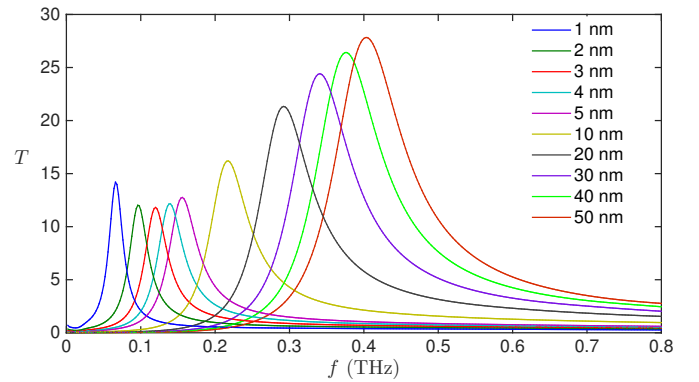
Fig. 9. Normalized transmission T for the TM polarization at various frequencies f and different gap sizes w . The incident angle \theta = 15^\circ .
