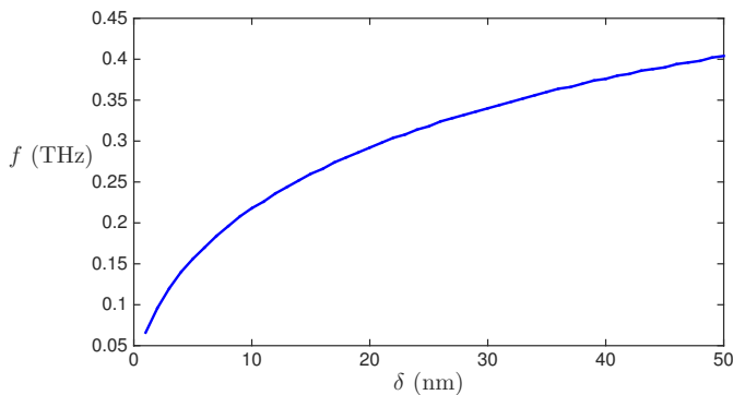
Fig. 13. Resonant frequencies for the TE polarization at different gap sizes w . The incident angle \theta = 15^\circ .
