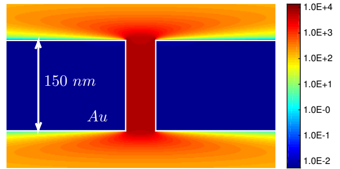
Fig. 5. Cross-sectional plot of |E_x| at the resonant frequency f = 0.156 THz on the xz plane when y = 0 . The gap width w = 5 nm.
