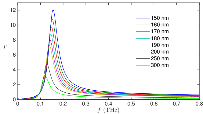
Fig. 8. Normalized transmission T for various frequencies f and different metal thicknesses d . The gap width w = 5 nm.
