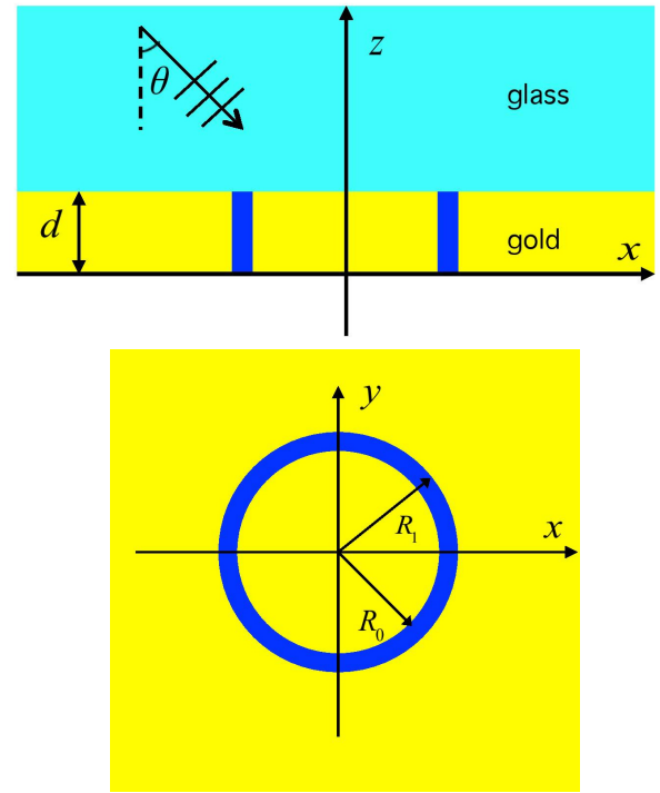
Fig. 1. Side view (top) and top view (bottom) of the nanostructure. The size of the annular gap w = R_1 - R_0 .
