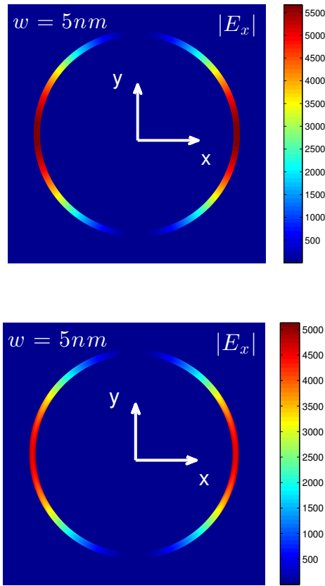
Fig. 4. Cross-sectional plot of |E_x| on the xy plane at the resonant frequency f = 0.156 THz: at z = 75 nm (top); (b) at z = 150.4 nm (bottom). The gap width w = 5 nm. The radial variable r is stretched to enlarge the annular gap in the figures.
