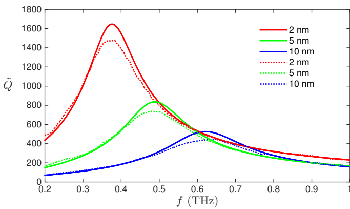
Fig. 15. The field enhancement factor \tilde{Q} obtained by the VMEM method for a single annular gap (solid lines) and by the HDG method for a periodic array of annular gaps (dotted lines).
