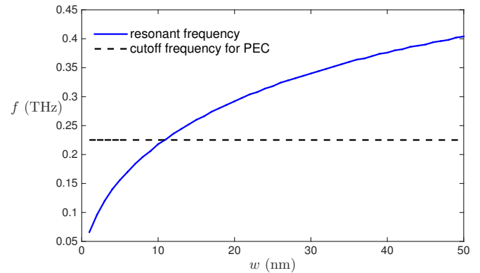
Fig. 6. Resonant frequencies for different gap sizes w . Note that the resonance frequency shifts from 0.156 THz to 0.06 THz as the gap width w decreases from 5 nm to 1 nm. For comparison, the cutoff frequencies for the PEC coaxial waveguide are also shown.
