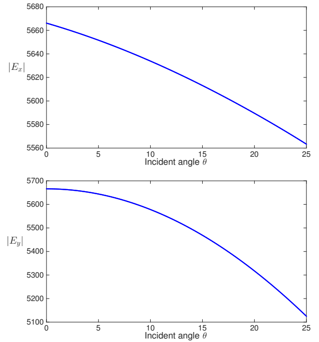
Fig. 14. |E_x| for the TM polarization (top) and |E_y| for the TE polarization (bottom) at the location (x, y, z) = (R_0 + w/2, 0, d/2) at the resonant frequencies for 0 < \theta < 25^\circ . The gap width w = 5 nm.
