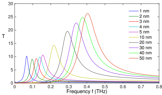
Fig. 12. Normalized transmission T for the TE polarization at various frequencies f and different gap sizes w . The incident angle \theta = 15^\circ .
