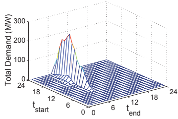
Fig. 1. Synthesized EV demand [22]. ( t_{\text{start}} : arrival time of an EV; t_{\text{end}} : departure time of an EV.)
