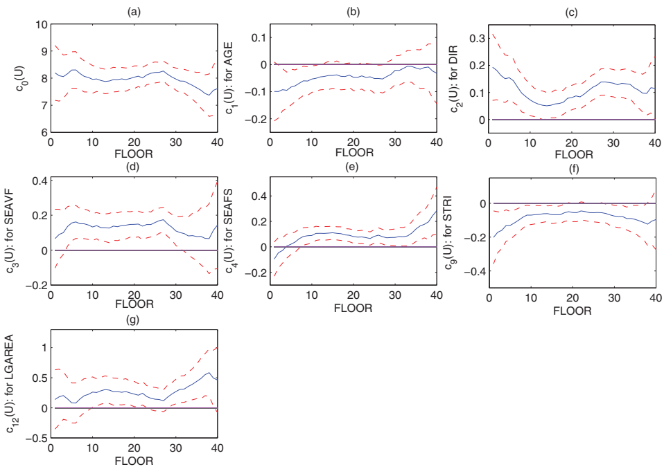
Figure 5. Plots of VC-QR estimated coefficient functions (solid curve) with 95% confidence interval (dashed curves) for \tau = 0.25 .
