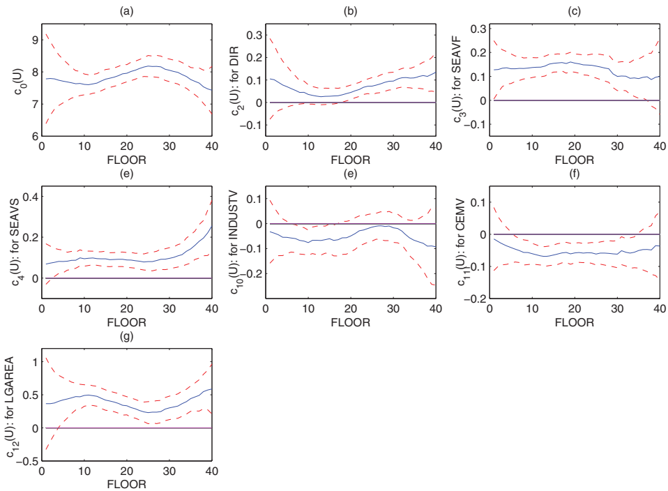
Figure 6. Plots of VC-QR estimated coefficient functions (solid curve) with 95% confidence interval (dashed curves) for \tau = 0.50 .
