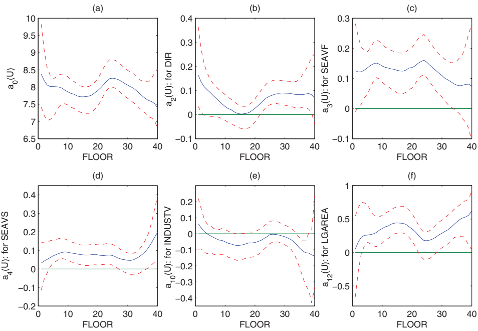
Figure 3. Plots of the estimated coefficient functions (solid curve) and the 95% simultaneous confidence bands (dashed curves) for estimated coefficient functions for the semi-VC model (12).
