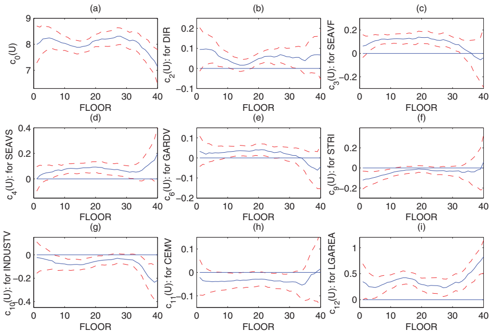
Figure 7. Plots of VC-QR estimated coefficient functions (solid curve) with 95% confidence interval (dashed curves) for \tau = 0.75 .
