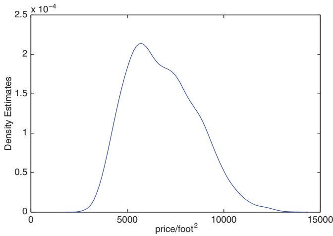
Figure 2. Estimated density of house prices.
