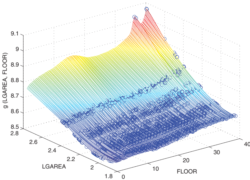
Figure 4. Surface plot of the estimated g(\cdot, \cdot) as a varying function of LGAREA and FLOOR.
