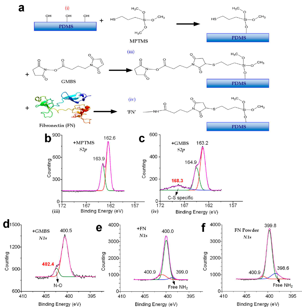
Figure 2. (a) Key chemical reactions at different steps in the ECM protein patterning based on covalently bonded molecules. (b–f) S 2p and N 1s XPS spectra at key steps in the covalent-bond method. All spectra were referenced to the C 1s peak of the PDMS substrate (284.8 eV). Deconvolutions were conducted to analyze the spectra.
